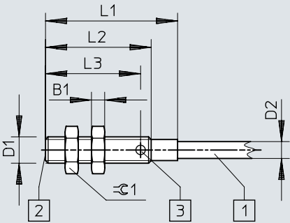
Dimensions – M5, flush mounted, cable
