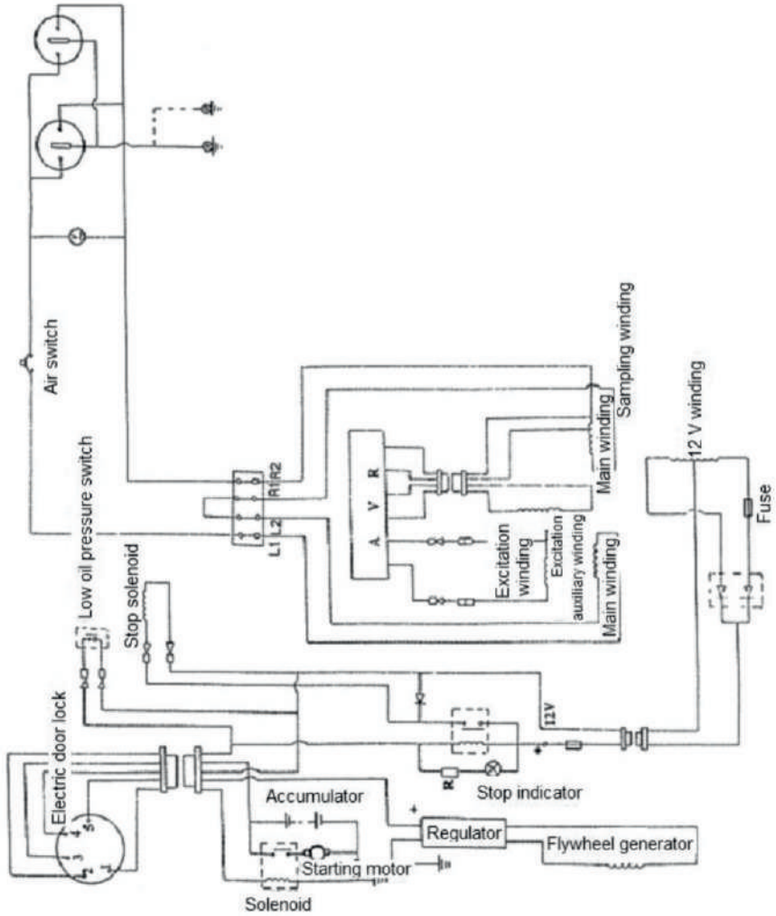
Electrical Wiring Diagram (Single Voltage Output)
