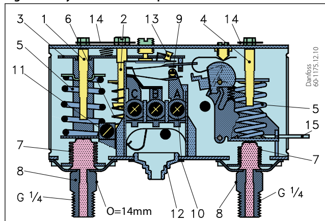
Figure 4: Key sketch of KP 44 pressure switch
