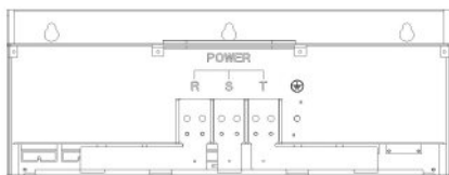
CV900G-350G/375P-14TF1 ~ CV900G-450G/500P-14TF1
